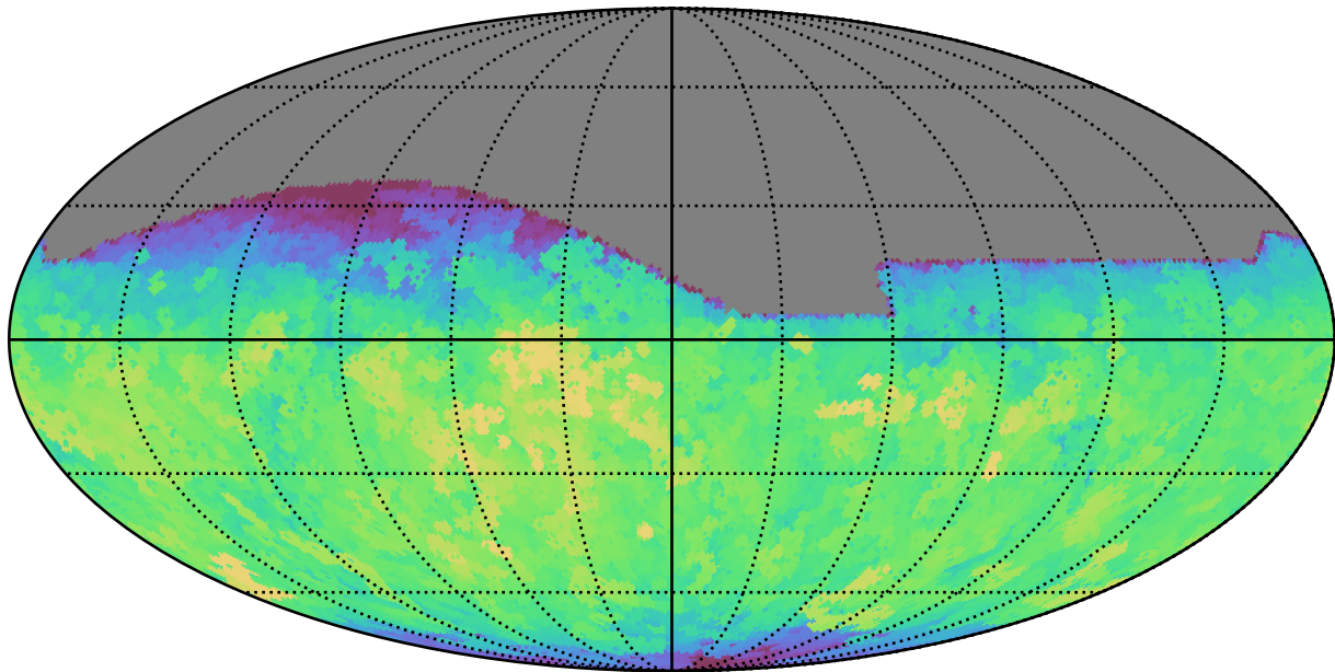
ddf_loaded_fl8_v3.4_10yrs All sky i band: Max saturation_mag
