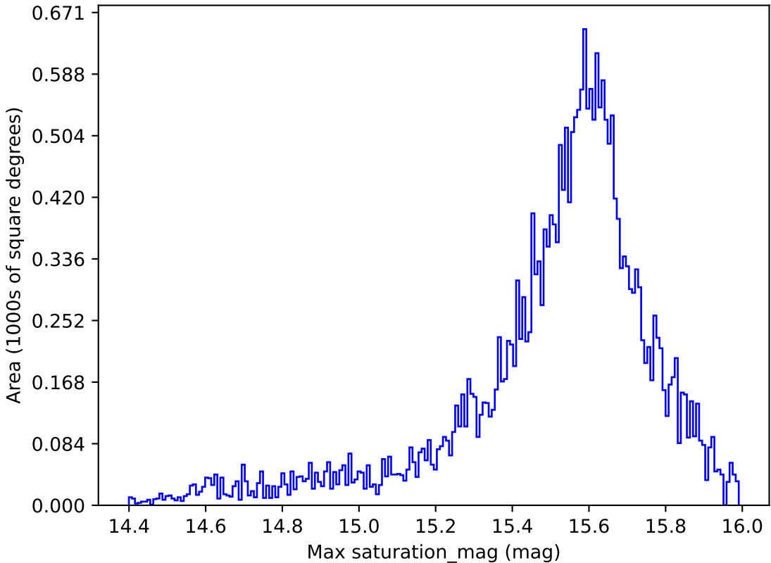
ddf_loaded_fl8_v3.4_10yrs All sky i band: Max saturation_mag
