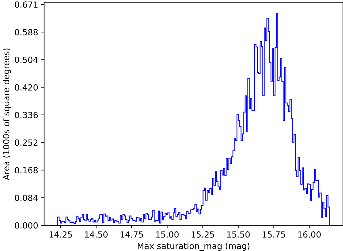
ddf_loaded_fl8_v3.4_10yrs All sky g band: Max saturation_mag
