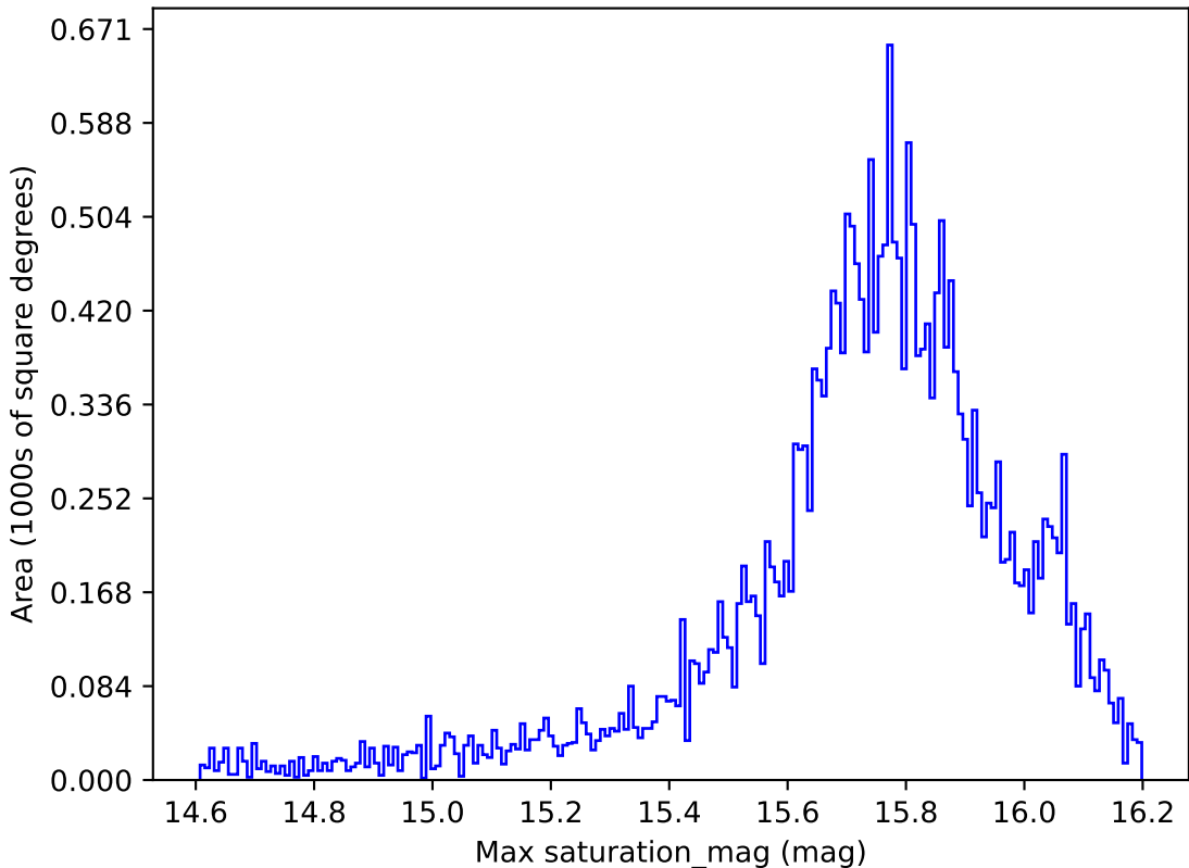
ddf_loaded_fl8_v3.4_10yrs All sky all bands: Max saturation_mag
