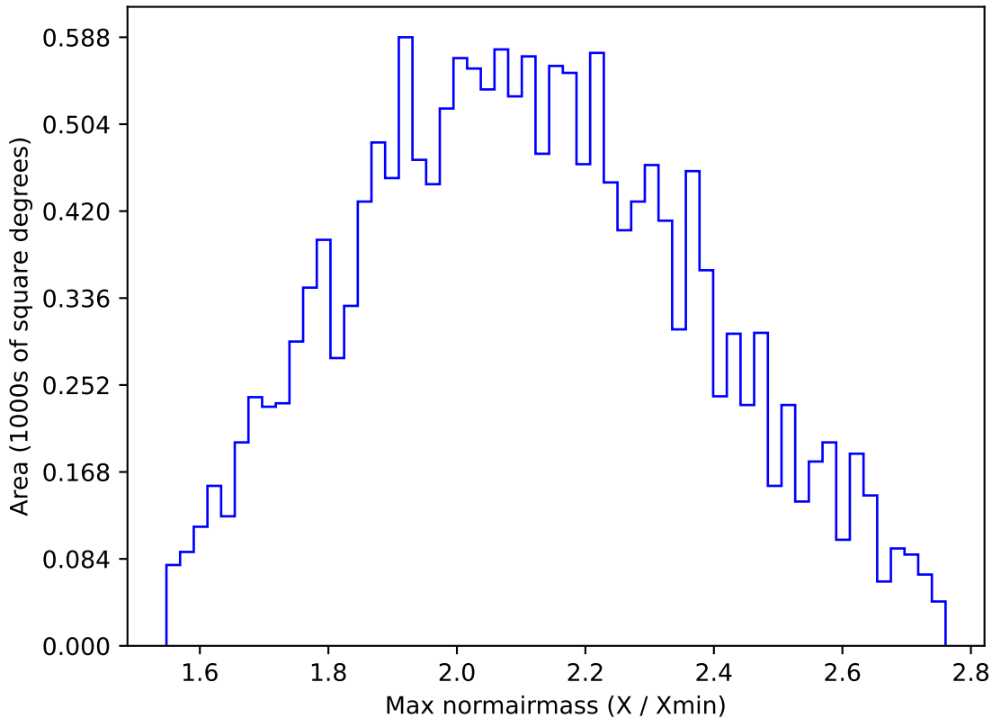
ddf_loaded_fl8_v3.4_10yrs WFD y band: Max normairmass
