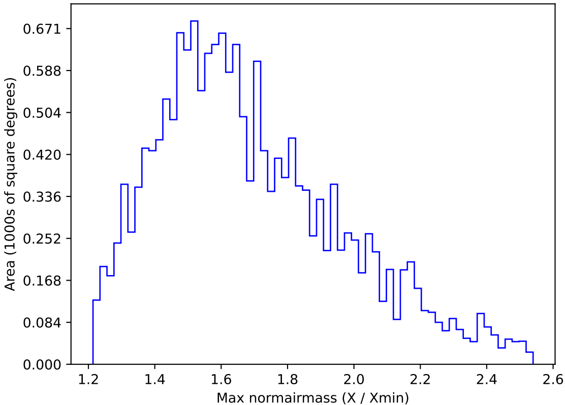
ddf_loaded_fl8_v3.4_10yrs WFD u band: Max normairmass
