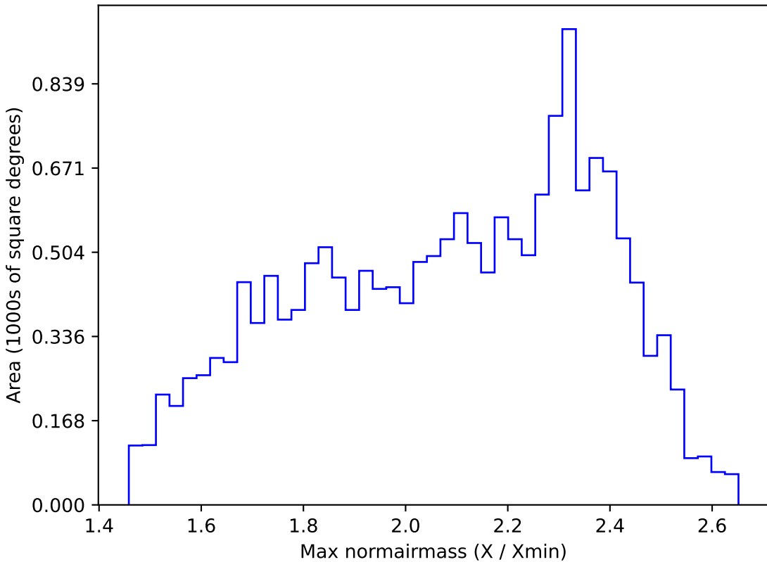
ddf_loaded_fl8_v3.4_10yrs WFD r band: Max normairmass
