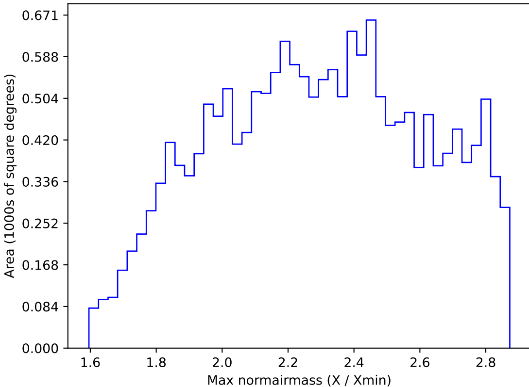
ddf_loaded_fl8_v3.4_10yrs WFD i band: Max normairmass
