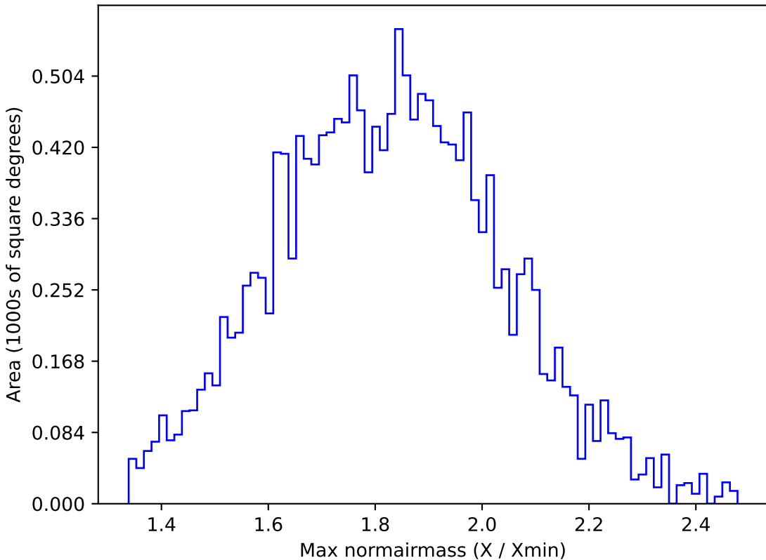
ddf_loaded_fl8_v3.4_10yrs WFD g band: Max normairmass
