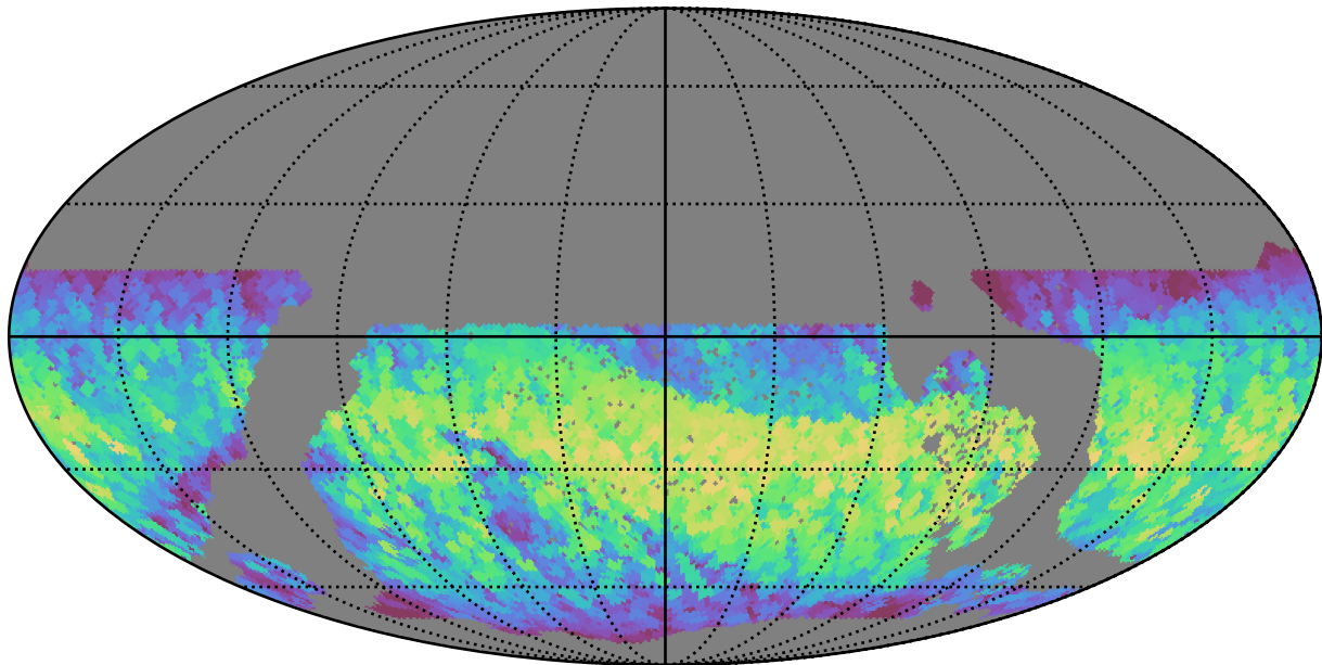
ddf_loaded_fl8_v3.4_10yrs WFD all bands: Max normairmass
