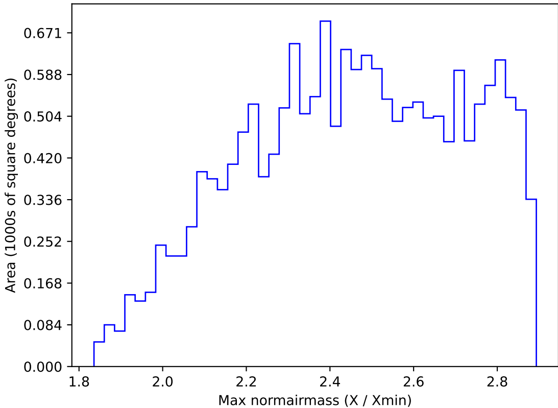
ddf_loaded_fl8_v3.4_10yrs WFD all bands: Max normairmass
