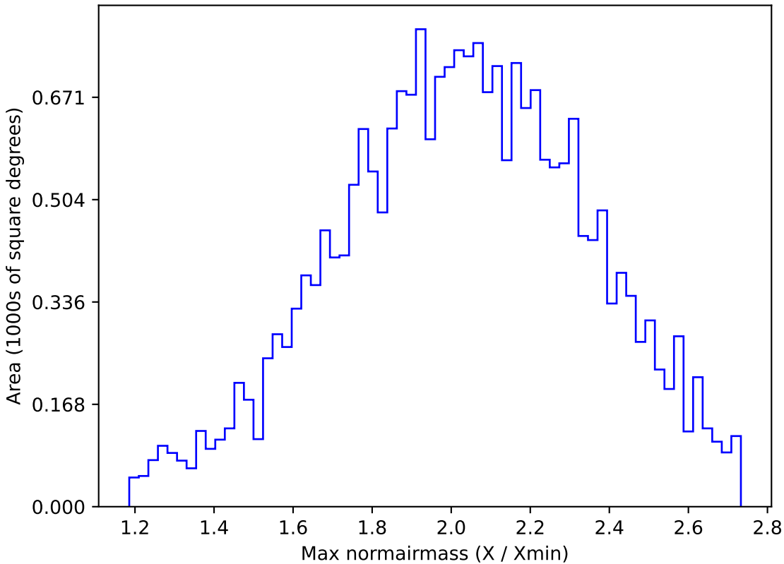
ddf_loaded_fl8_v3.4_10yrs All sky y band: Max normairmass
