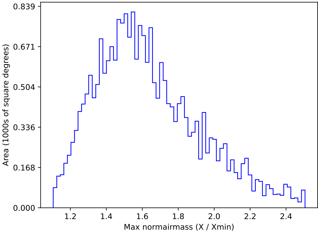
ddf_loaded_fl8_v3.4_10yrs All sky u band: Max normairmass
