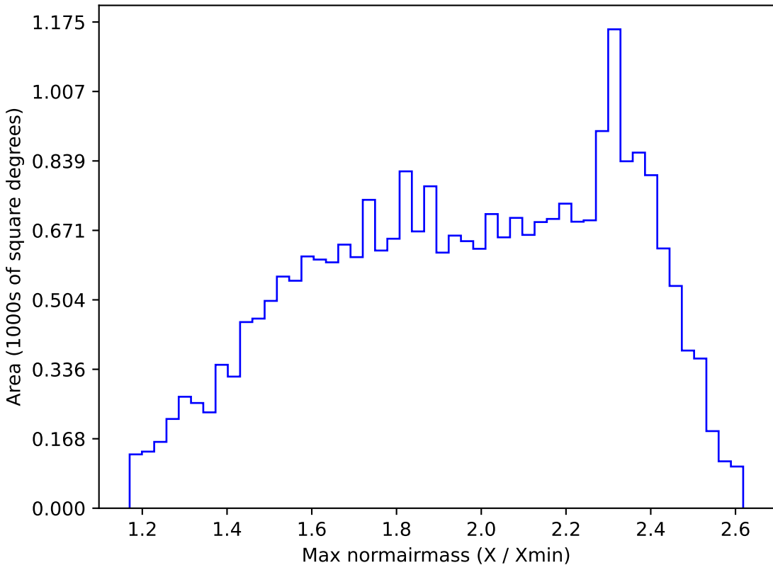
ddf_loaded_fl8_v3.4_10yrs All sky r band: Max normairmass
