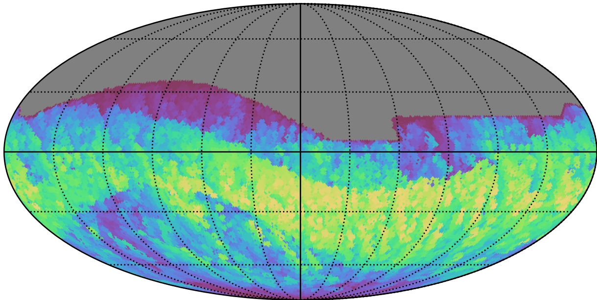
ddf_loaded_fl8_v3.4_10yrs All sky i band: Max normairmass
