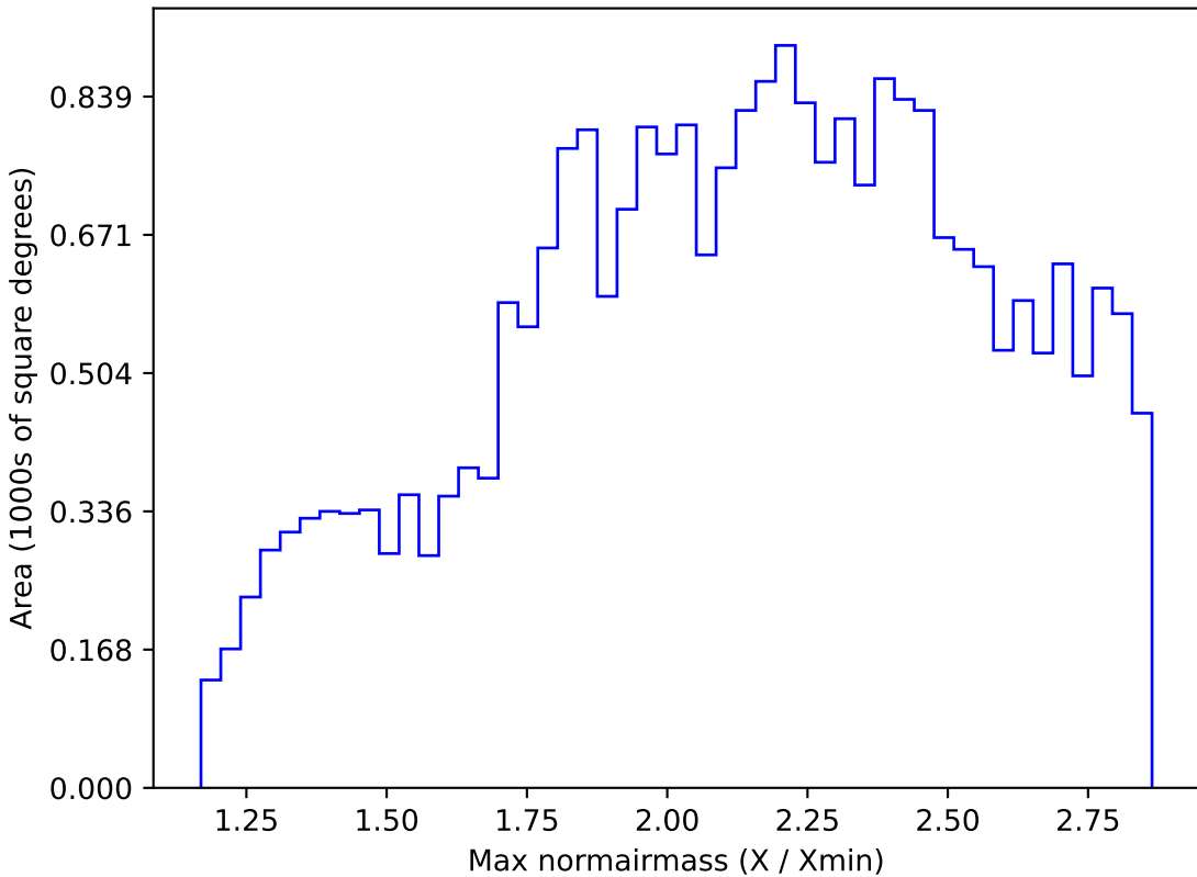
ddf_loaded_fl8_v3.4_10yrs All sky i band: Max normairmass
