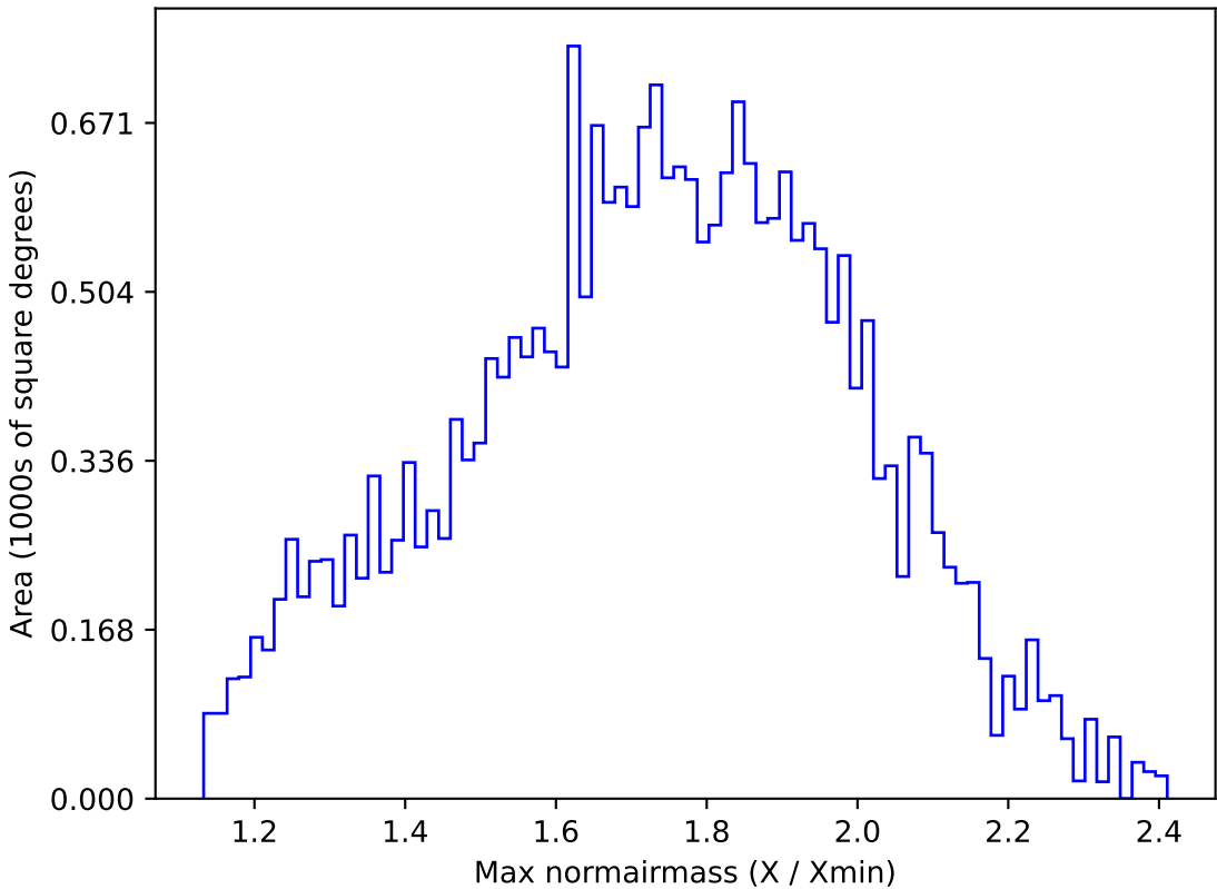
ddf_loaded_fl8_v3.4_10yrs All sky g band: Max normairmass
