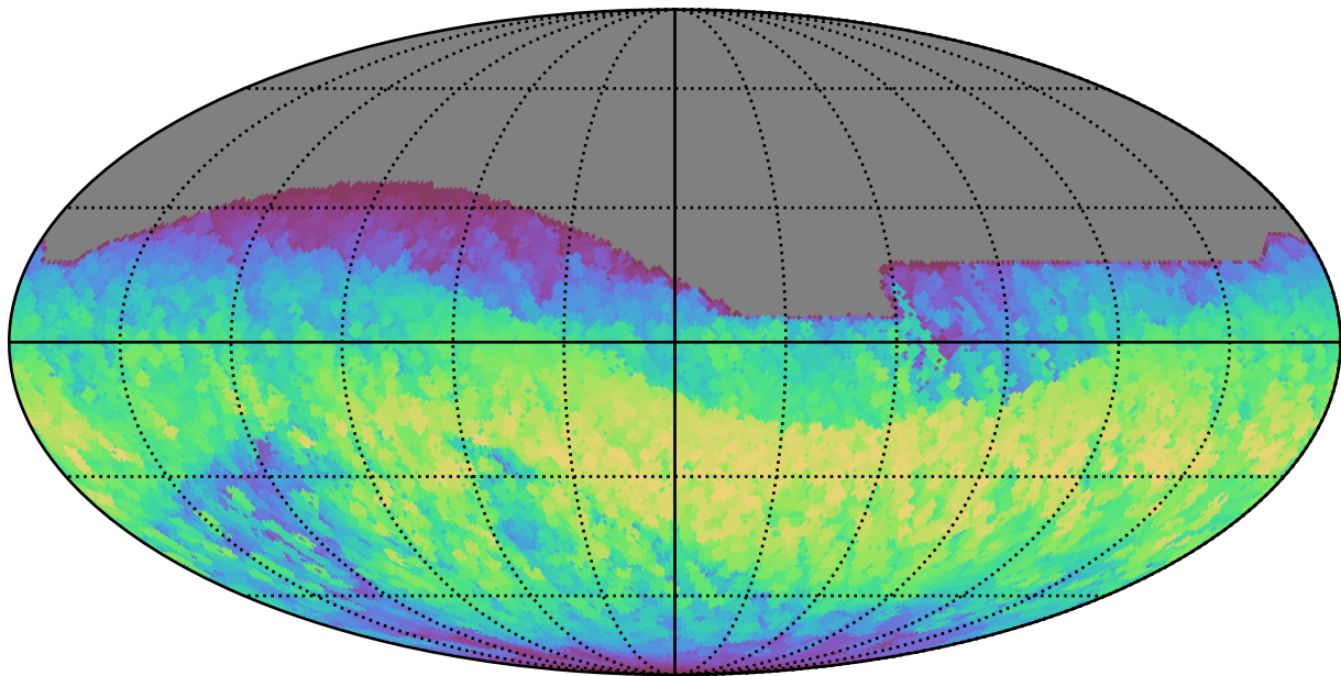
ddf_loaded_fl8_v3.4_10yrs All sky all bands: Max normairmass
