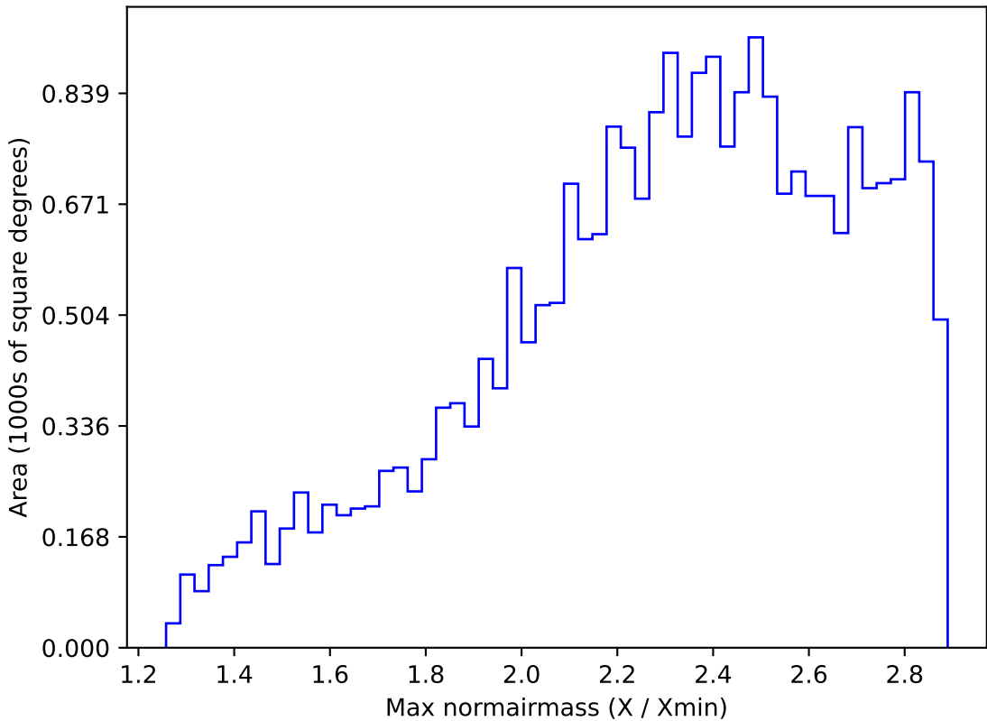
ddf_loaded_fl8_v3.4_10yrs All sky all bands: Max normairmass
