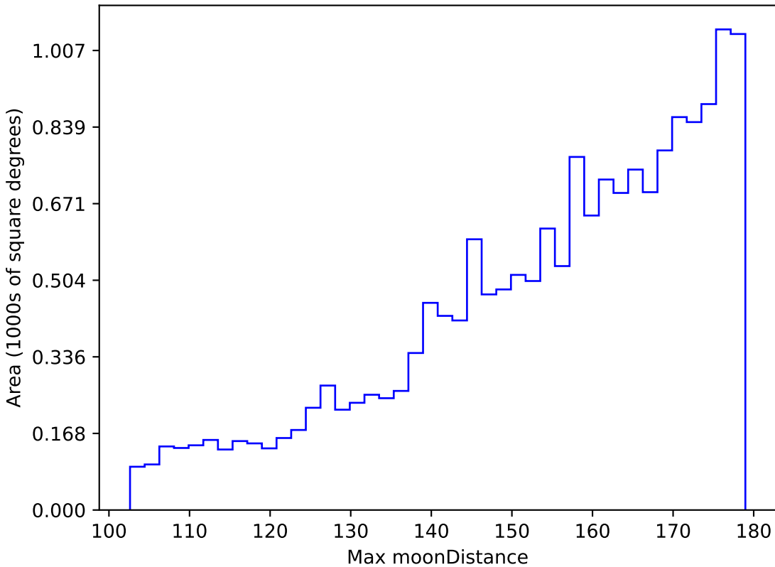
ddf_loaded_fl8_v3.4_10yrs WFD z band: Max moonDistance
