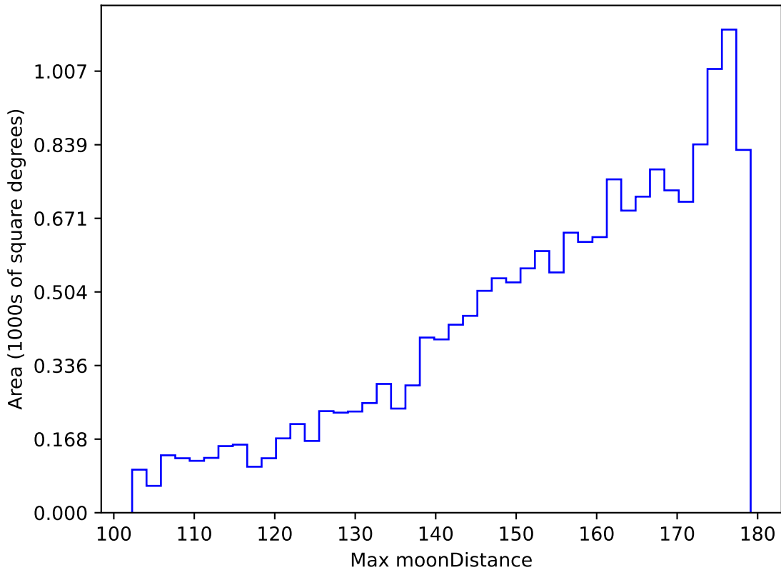
ddf_loaded_fl8_v3.4_10yrs WFD u band: Max moonDistance
