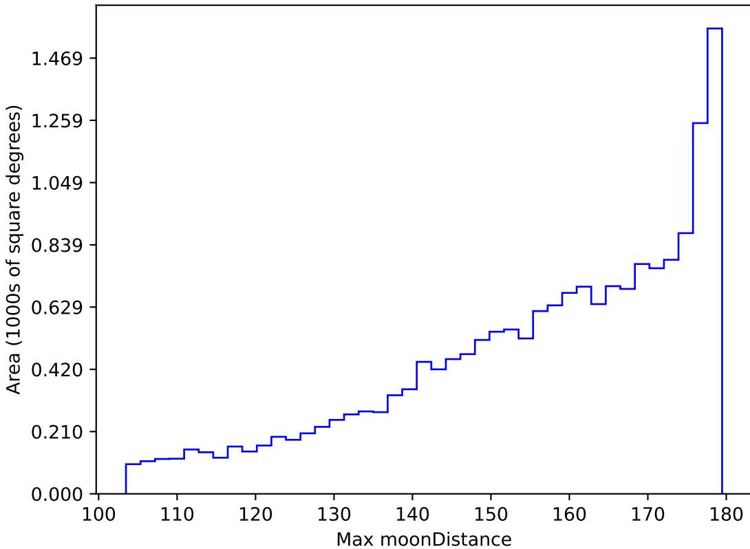
ddf_loaded_fl8_v3.4_10yrs WFD r band: Max moonDistance
