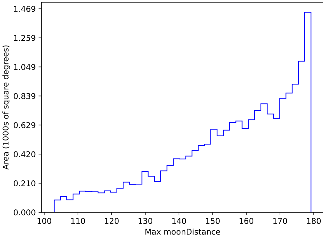
ddf_loaded_fl8_v3.4_10yrs WFD i band: Max moonDistance
