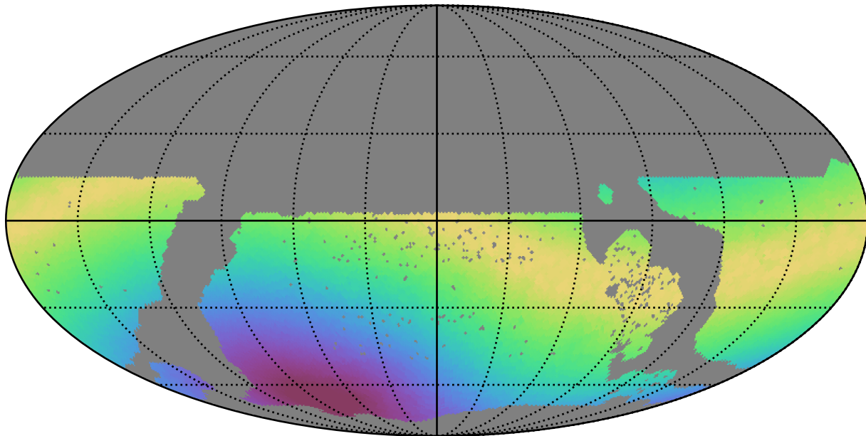
ddf_loaded_fl8_v3.4_10yrs WFD all bands: Max moonDistance
