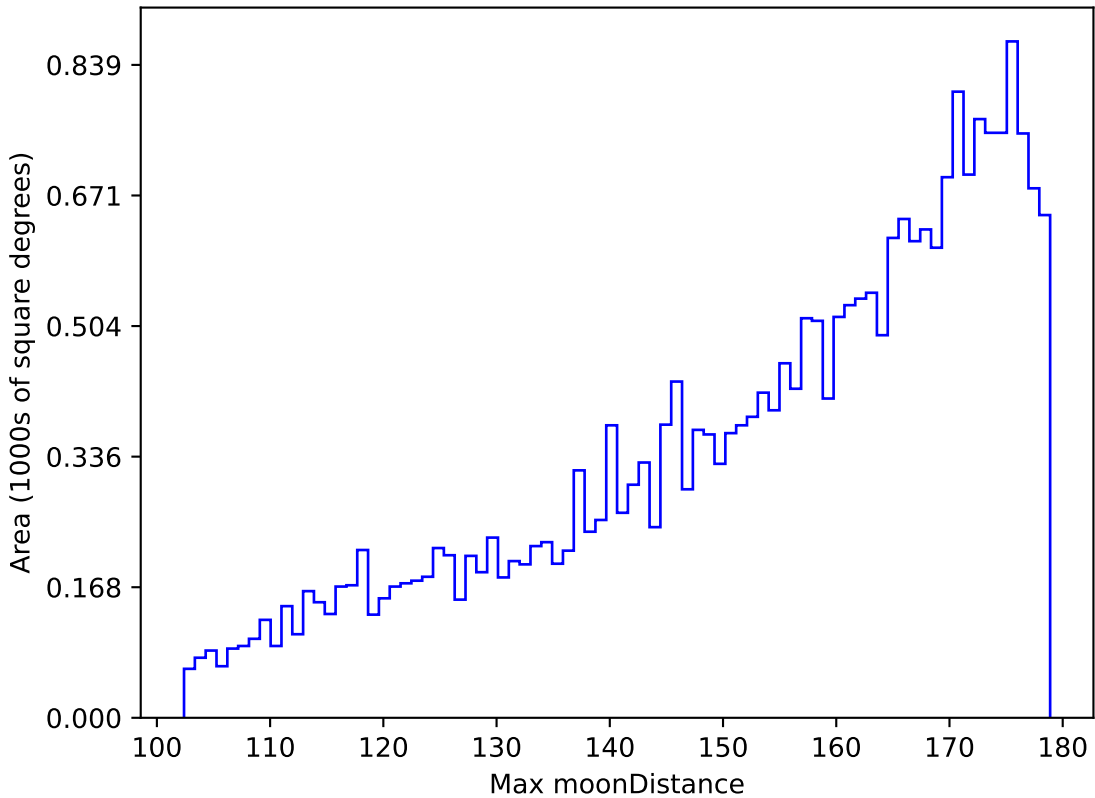
ddf_loaded_fl8_v3.4_10yrs All sky z band: Max moonDistance
