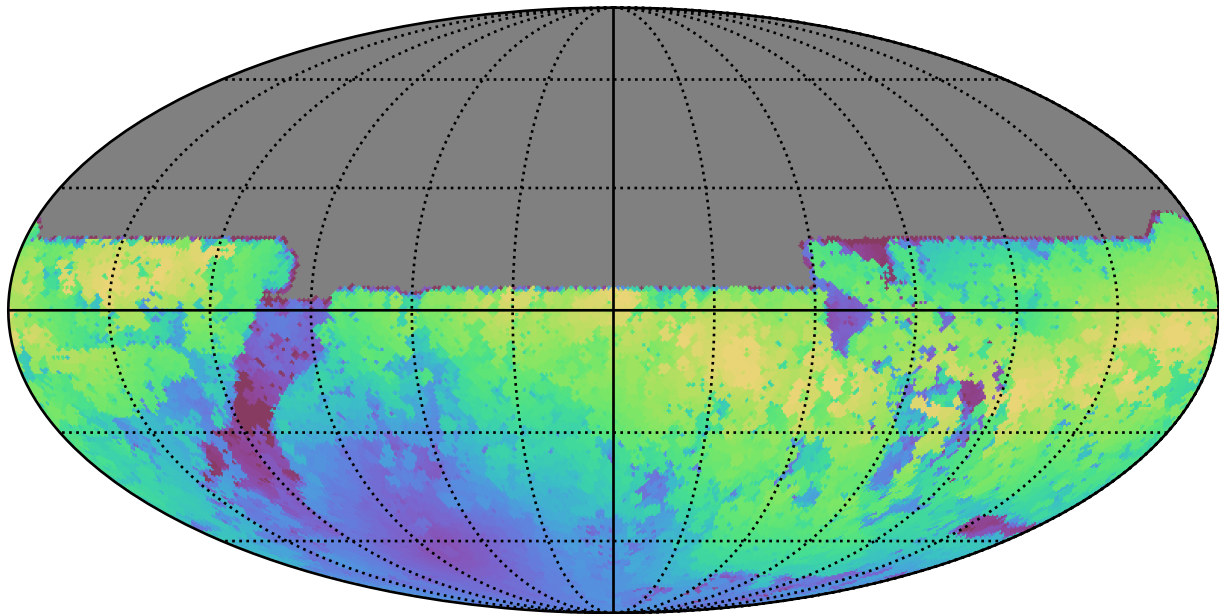
ddf_loaded_fl8_v3.4_10yrs All sky y band: Max moonDistance
