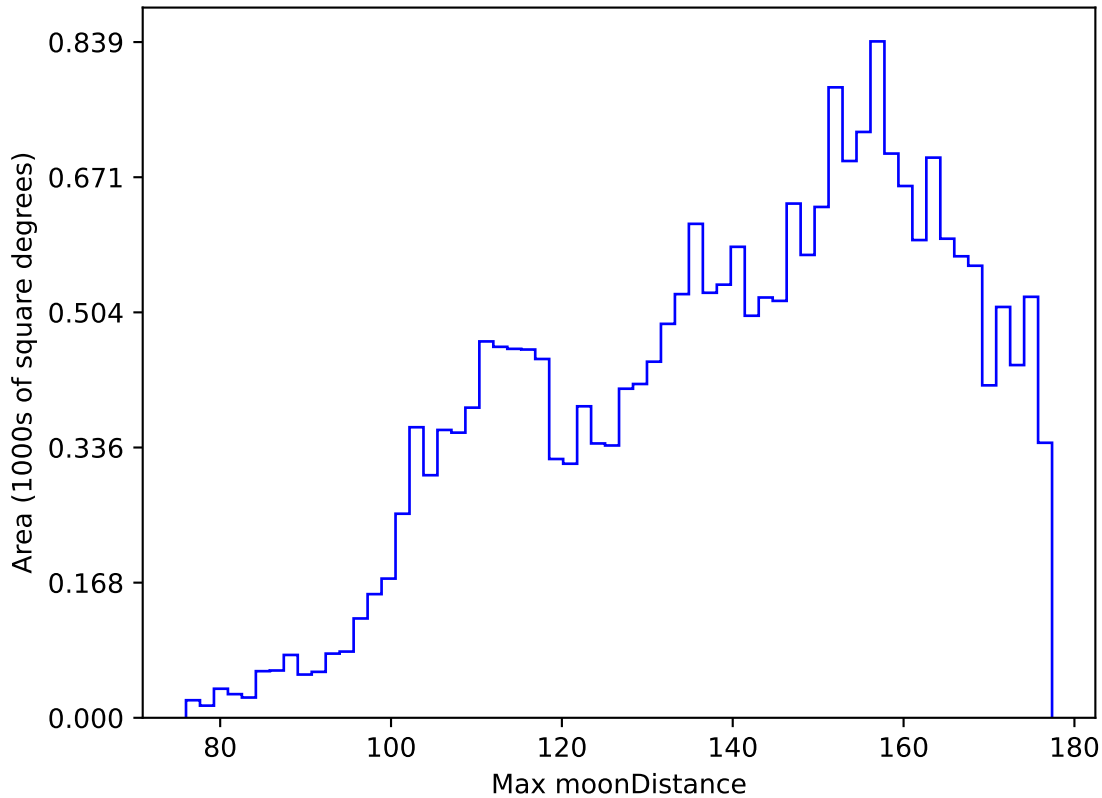
ddf_loaded_fl8_v3.4_10yrs All sky y band: Max moonDistance
