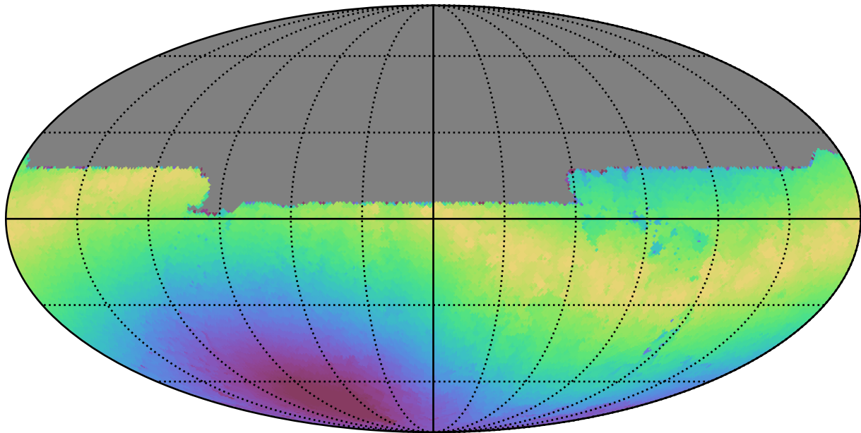
ddf_loaded_fl8_v3.4_10yrs All sky u band: Max moonDistance
