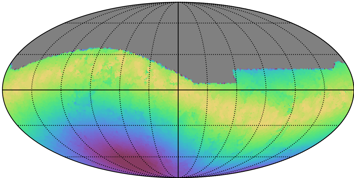
ddf_loaded_fl8_v3.4_10yrs All sky g band: Max moonDistance
