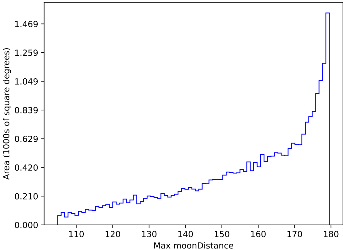
ddf_loaded_fl8_v3.4_10yrs All sky all bands: Max moonDistance
