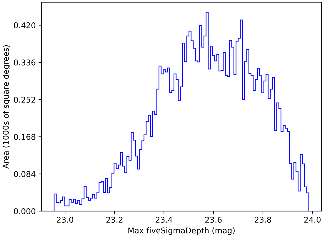
ddf_loaded_fl8_v3.4_10yrs Yr 1 u band: Max fiveSigmaDepth
