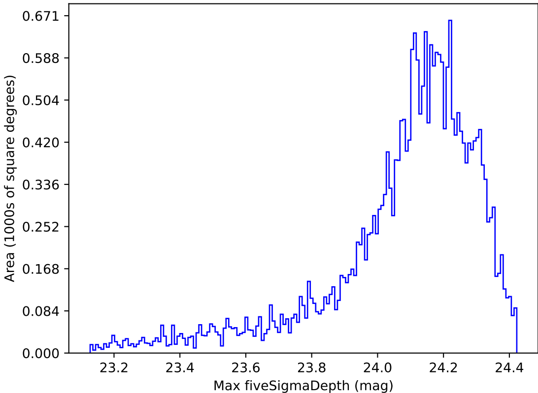
ddf_loaded_fl8_v3.4_10yrs Yr 1 i band: Max fiveSigmaDepth
