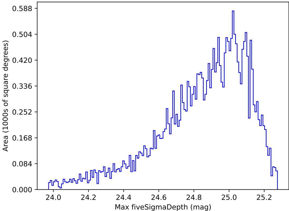
ddf_loaded_fl8_v3.4_10yrs Yr 1 g band: Max fiveSigmaDepth
