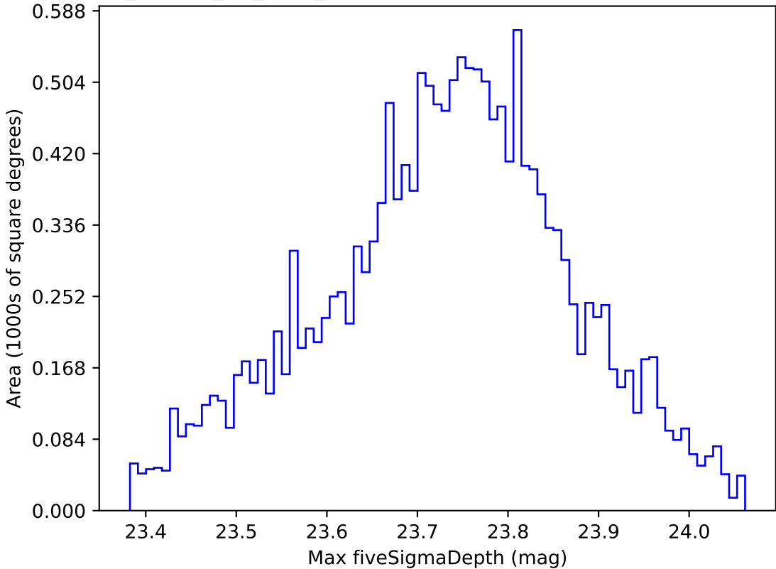
ddf_loaded_fl8_v3.4_10yrs WFD u band: Max fiveSigmaDepth
