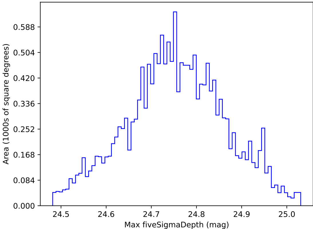
ddf_loaded_fl8_v3.4_10yrs WFD r band: Max fiveSigmaDepth
