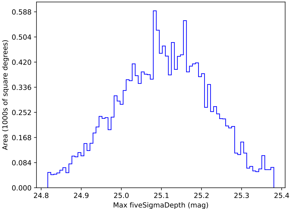
ddf_loaded_fl8_v3.4_10yrs WFD g band: Max fiveSigmaDepth
