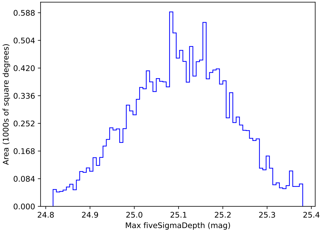
ddf_loaded_fl8_v3.4_10yrs WFD all bands: Max fiveSigmaDepth
