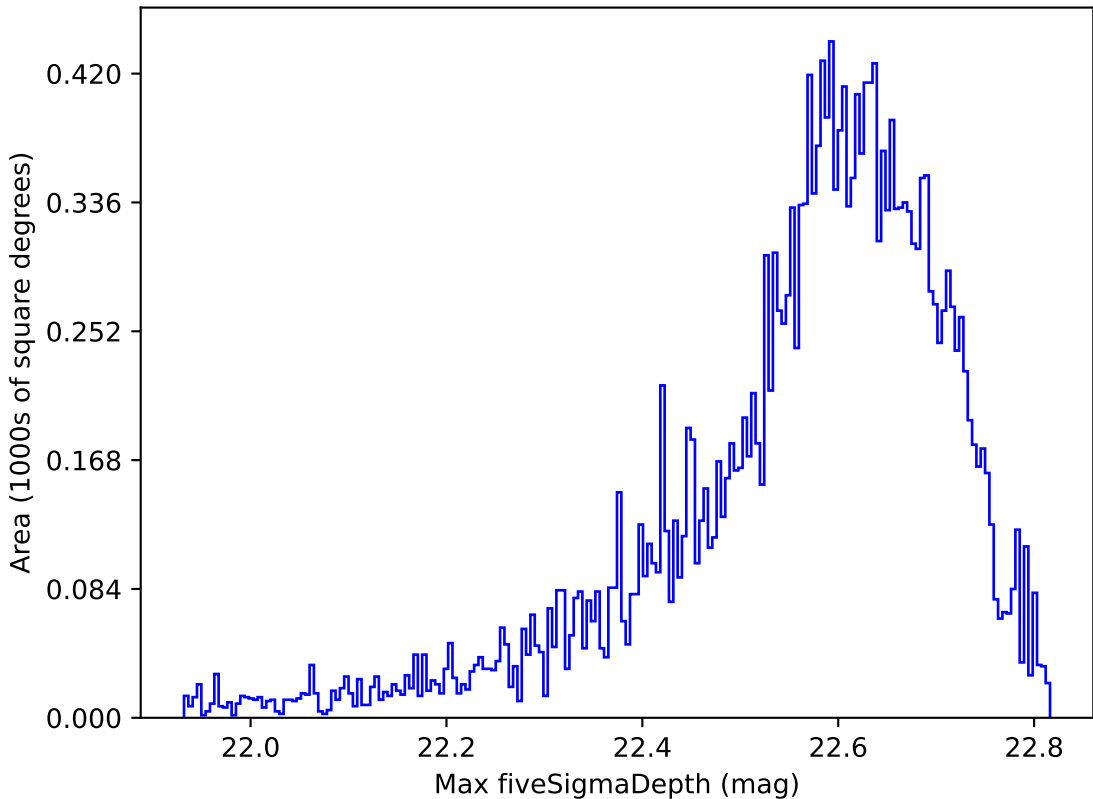
ddf_loaded_fl8_v3.4_10yrs All sky y band: Max fiveSigmaDepth
