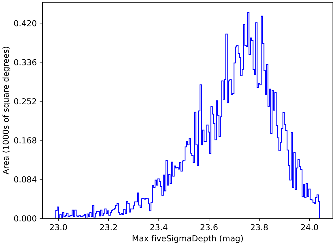
ddf_loaded_fl8_v3.4_10yrs All sky u band: Max fiveSigmaDepth
