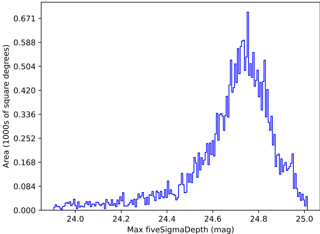
ddf_loaded_fl8_v3.4_10yrs All sky r band: Max fiveSigmaDepth
