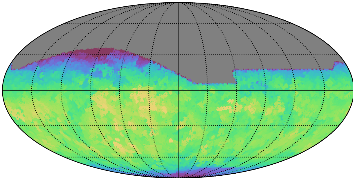
ddf_loaded_fl8_v3.4_10yrs All sky i band: Max fiveSigmaDepth
