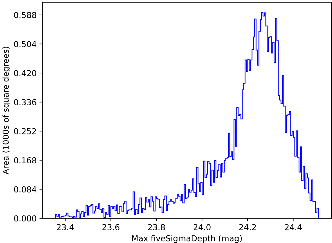
ddf_loaded_fl8_v3.4_10yrs All sky i band: Max fiveSigmaDepth
