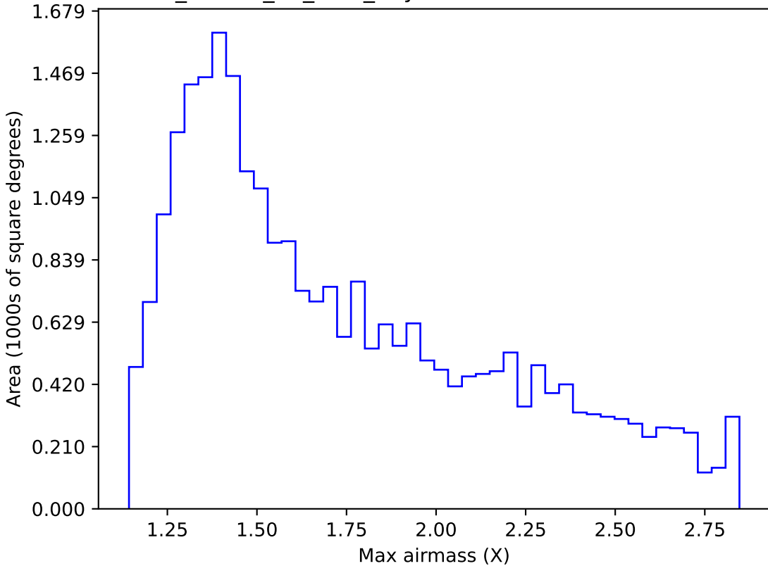
ddf_loaded_fl8_v3.4_10yrs Yr 1 z band: Max airmass
