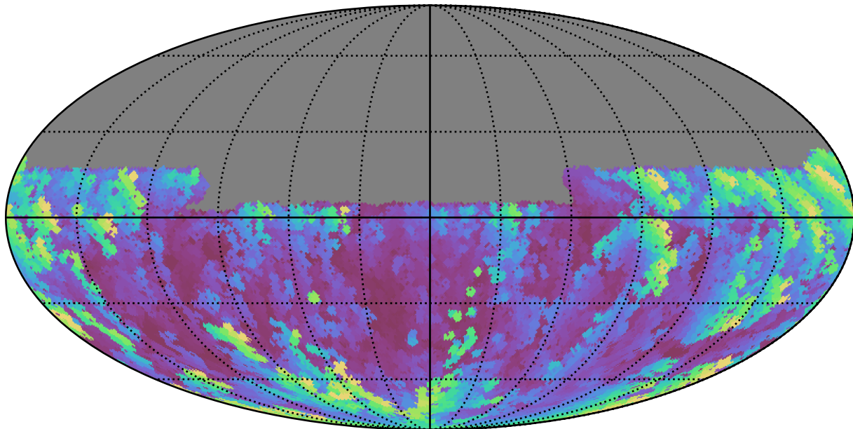
ddf_loaded_fl8_v3.4_10yrs Yr 1 y band: Max airmass
