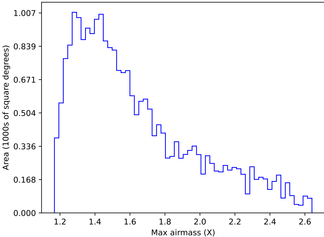
ddf_loaded_fl8_v3.4_10yrs Yr 1 y band: Max airmass
