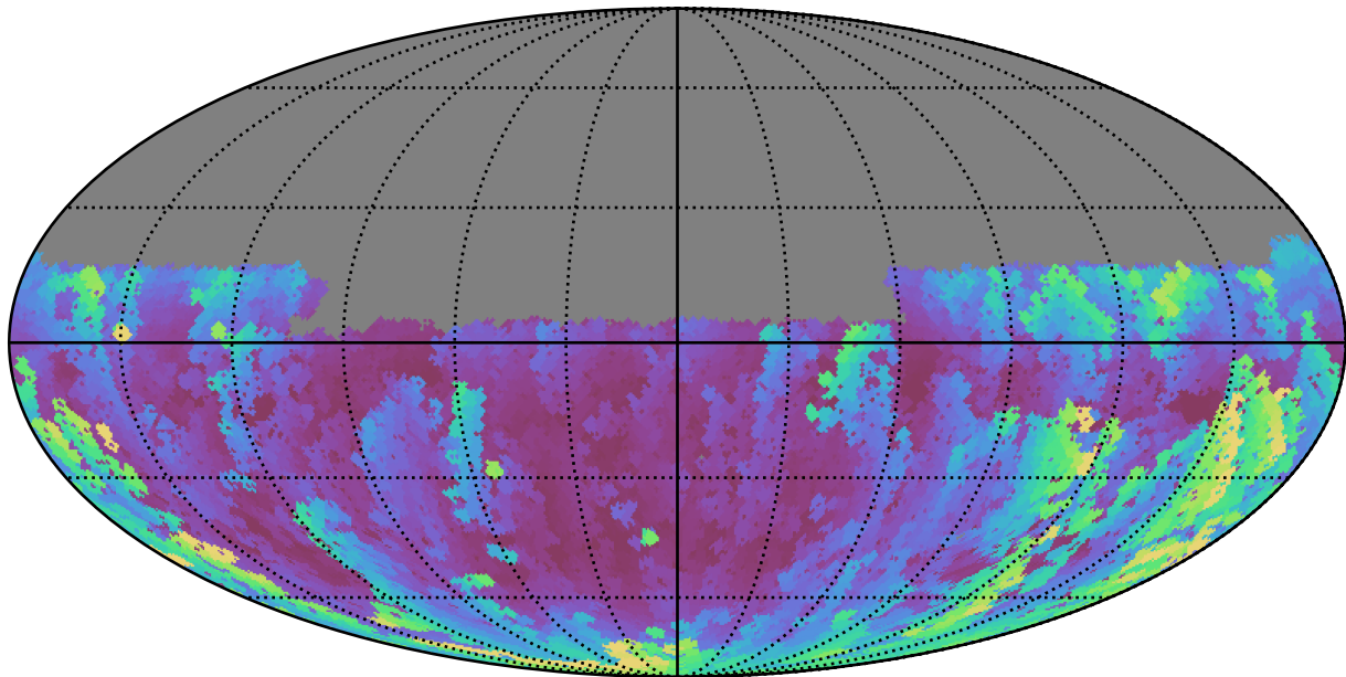
ddf_loaded_fl8_v3.4_10yrs Yr 1 u band: Max airmass
