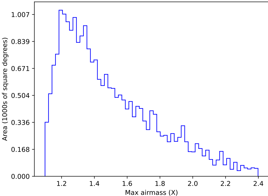
ddf_loaded_fl8_v3.4_10yrs Yr 1 u band: Max airmass
