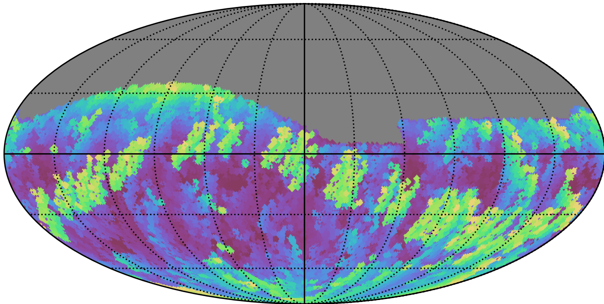
ddf_loaded_fl8_v3.4_10yrs Yr 1 r band: Max airmass
