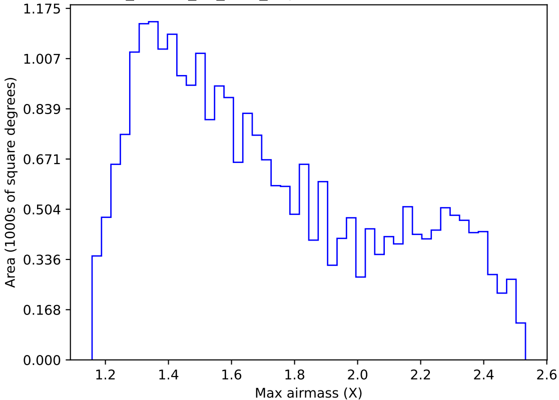
ddf_loaded_fl8_v3.4_10yrs Yr 1 r band: Max airmass
