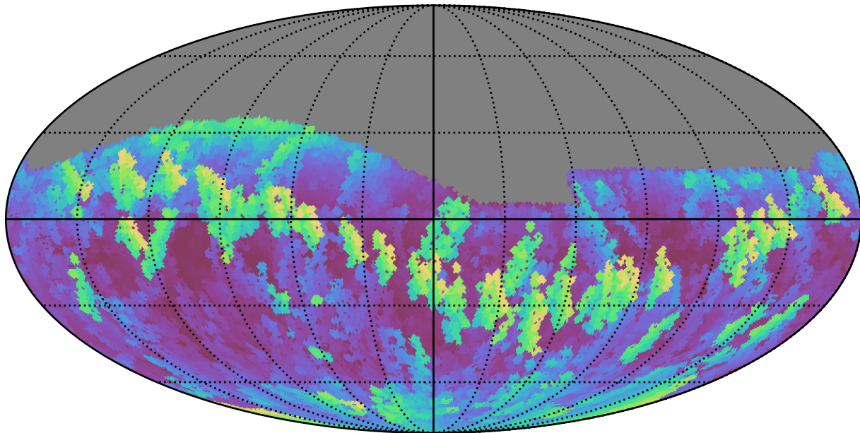
ddf_loaded_fl8_v3.4_10yrs Yr 1 i band: Max airmass
